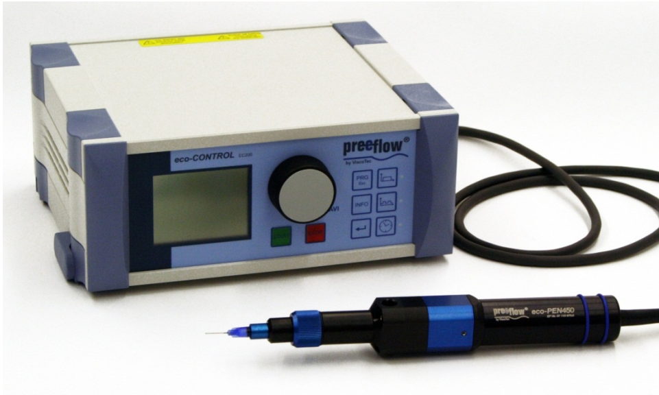
Figure 5 – Endless-Piston-Principle technology in a pen, with digital controller
